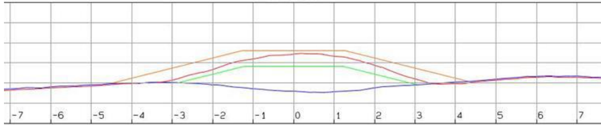
SECTION B, 1 : 5 COVER LAYER: SURFACE LAID/EXPOSED CABLE
