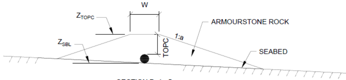
SECTION B, 1 : 5 COVER LAYER: SURFACE LAID/EXPOSED CABLE
